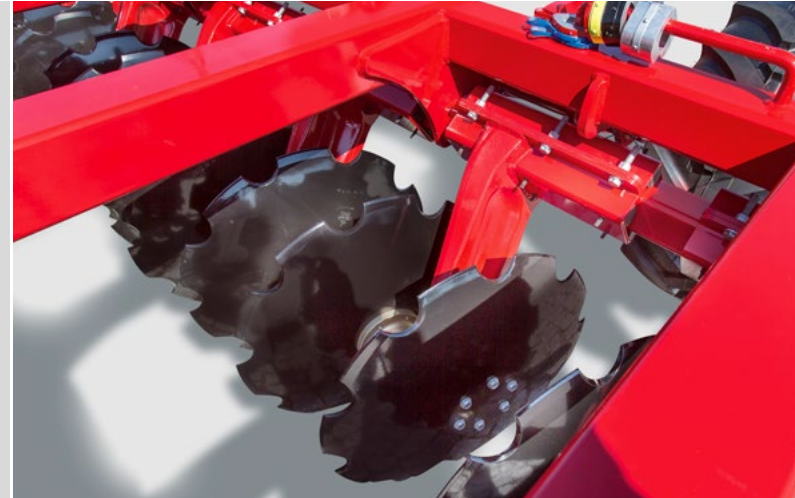
Large (Ø 62 cm) discs for working deeply
